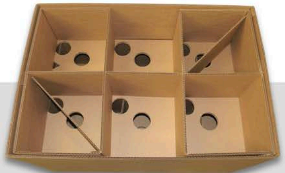
Custom corrugated paper partition with part positioning cuts
